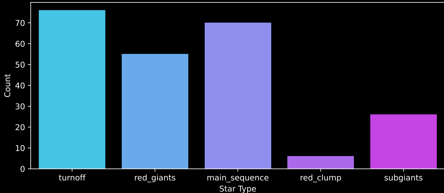
GALAH DR4 Field: [7194] Count plot of Star Type
