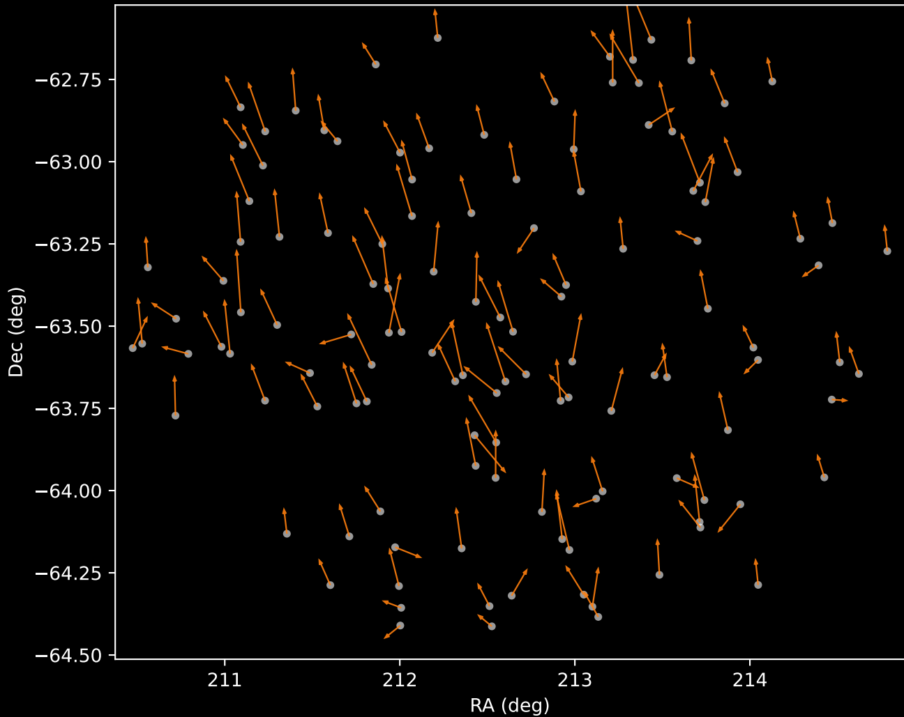
GALAH DR4 Cluster 2 Proper Motion Vectors (n=124)
