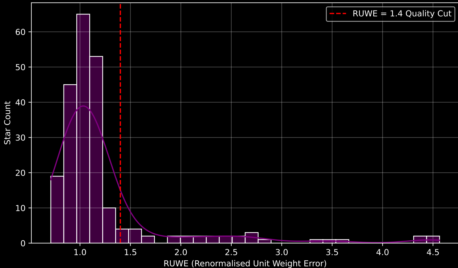
GALAH DR4 Field [7194] RUWE Distribution (n= 225)
