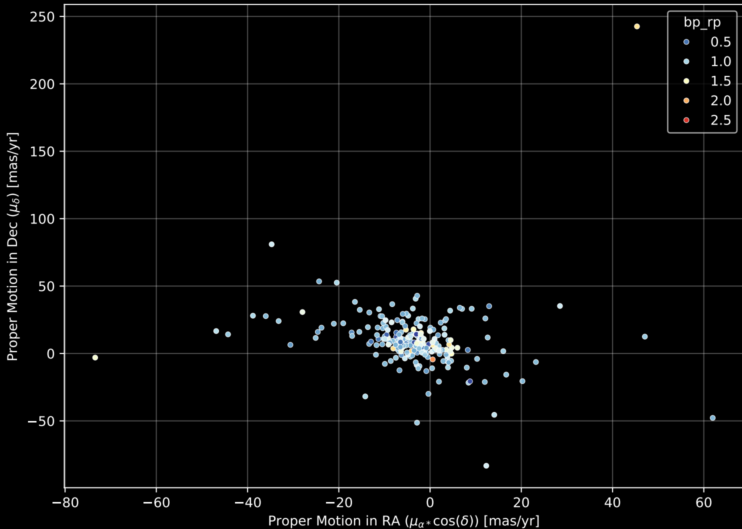
GALAH DR4 Field: [7194] Proper Motion Diagram (n= 233)
